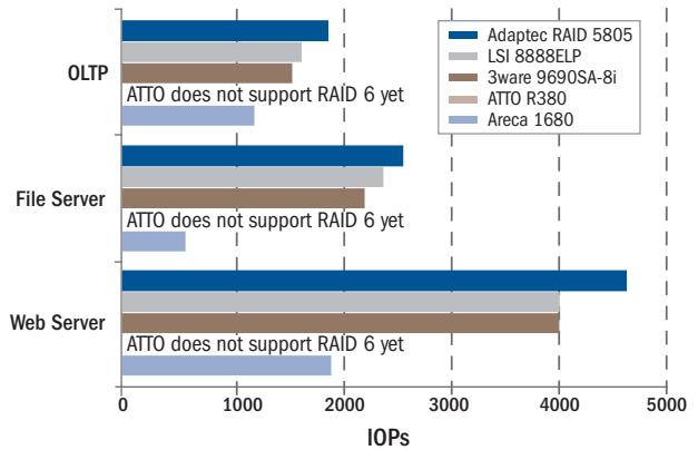
Figure 4. Sixteen-drive competitive workloads performance comparison for Adaptec RAID 5805, 3ware 9690SA-8i, LSI 8888ELP, ATTO R380, and Areca 1680 using sixteen 15K RPM Seagate SAS disk drives in a cache enabled high-availability RAID 6 array. ATTO does not support RAID 6.
