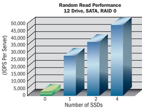
Figure 8: Using Adaptec 5805Q, with 100GB SSDs, 12 SATA HDDs, at 512K block size
