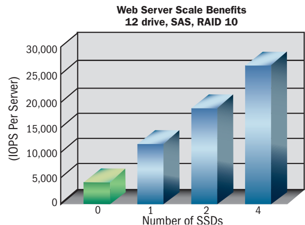
Figure 2: Using Adaptec 5805Q, with 100GB SSDs, 12 SATA HDDs, at 512K block size
