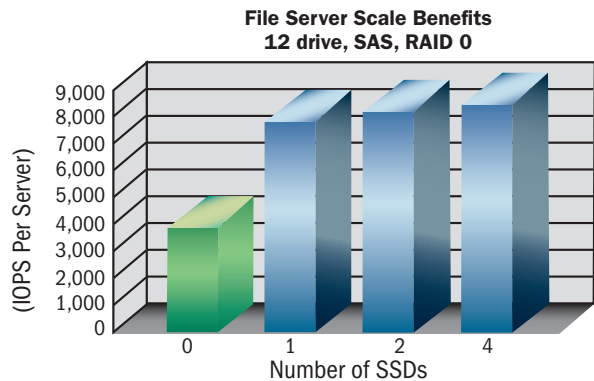
Figure 3: Using Adaptec 5805Q, with 100GB SSDs, 12 SATA HDDs, at 512K block size
