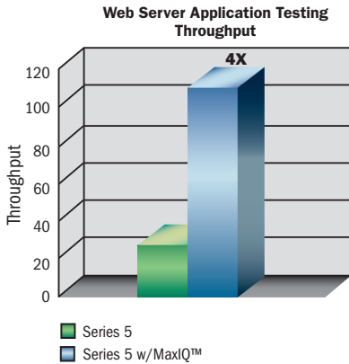
Figure 7: SSD Caching
